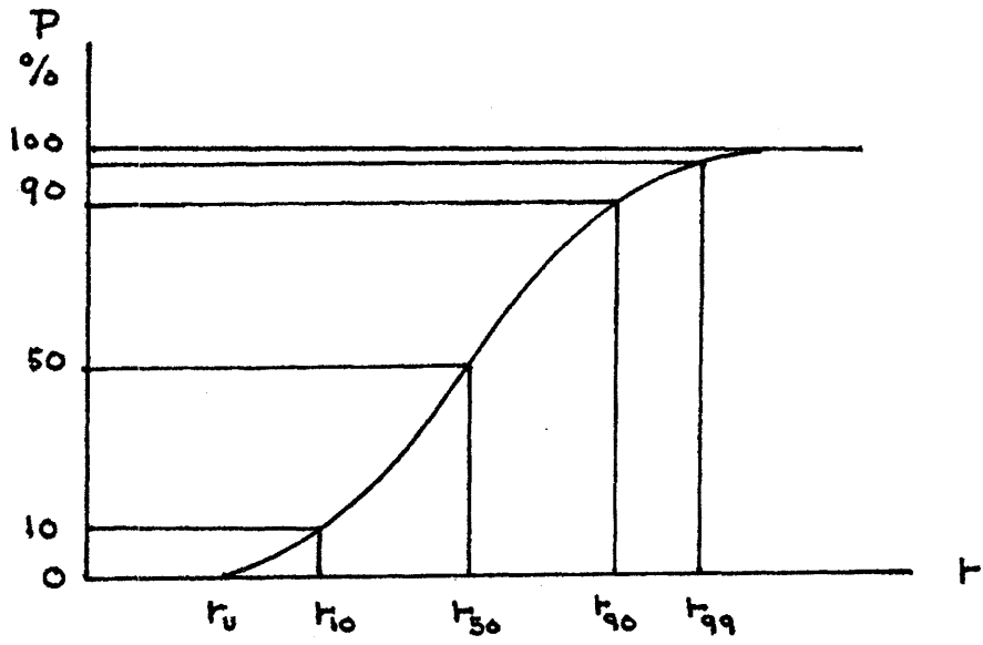
FIGURE 1. THE DISTRIBUTION FUNCTION F(r) .
