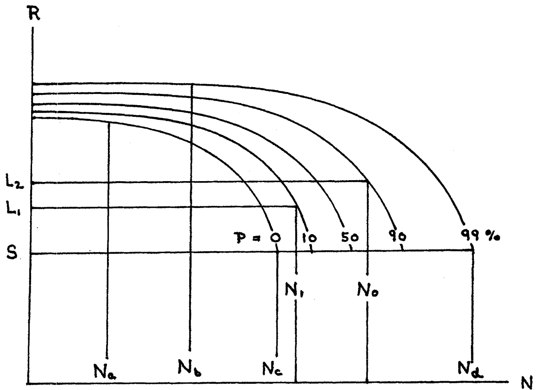
FIGURE 1. THE DISTRIBUTION FUNCTION F(r) .
