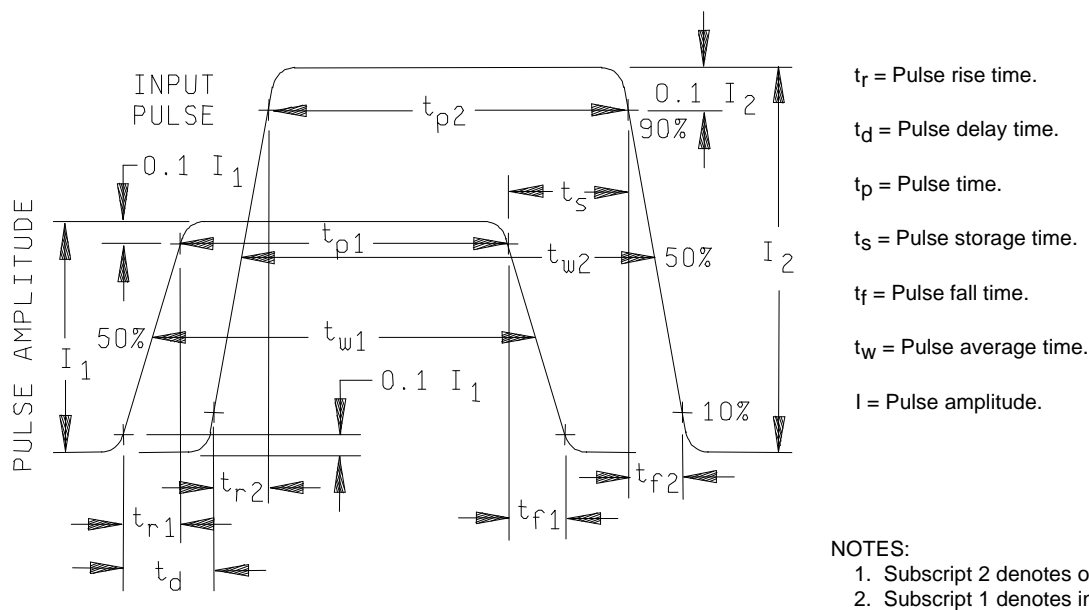
FIGURE 1. Pulse measurements .
